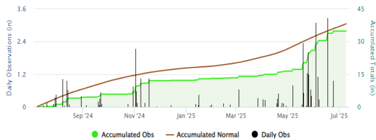
Elmdale 1SE 365 Day Accumulated Precipitation
