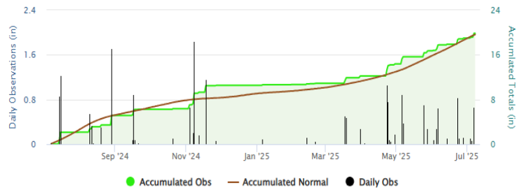
Garden City 365 Day Accumulated Precipitation
