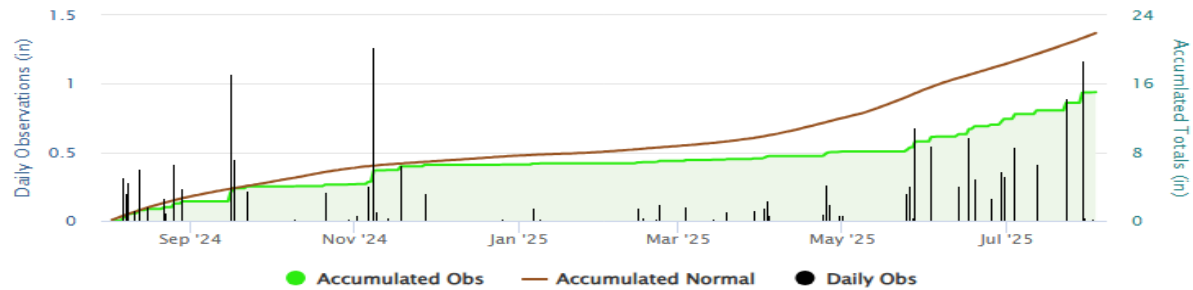
Oberlin 7NE 365 Day Accumulated Precipitation
