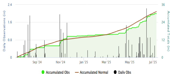
Gypsum 365 Day Accumulated Precipitation
